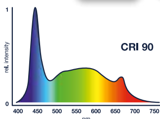
Spectre de couleurs classicLED plants
